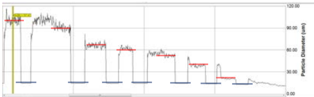
Figure 1: Online measurements of Dv50 upstream and downstream a valve
